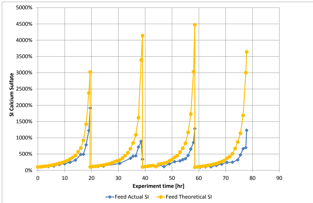
Figure 5: Calcium Sulphate Saturation Index Changes during the Pilot study
