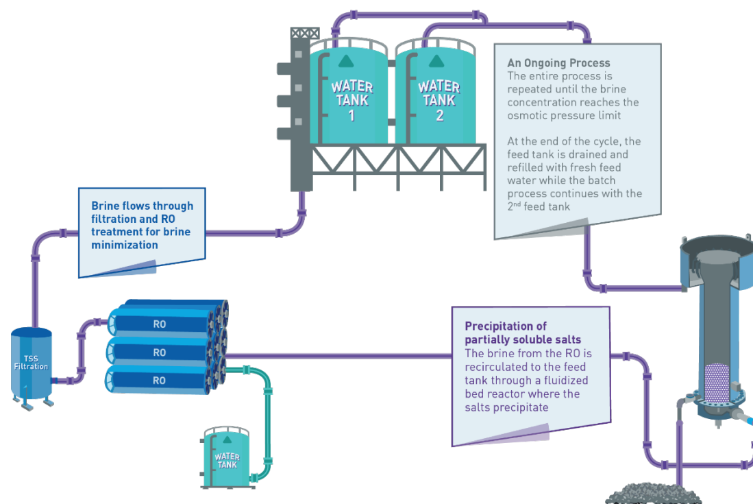
Figure 1: The Brine Minimization Technology Process Scheme
