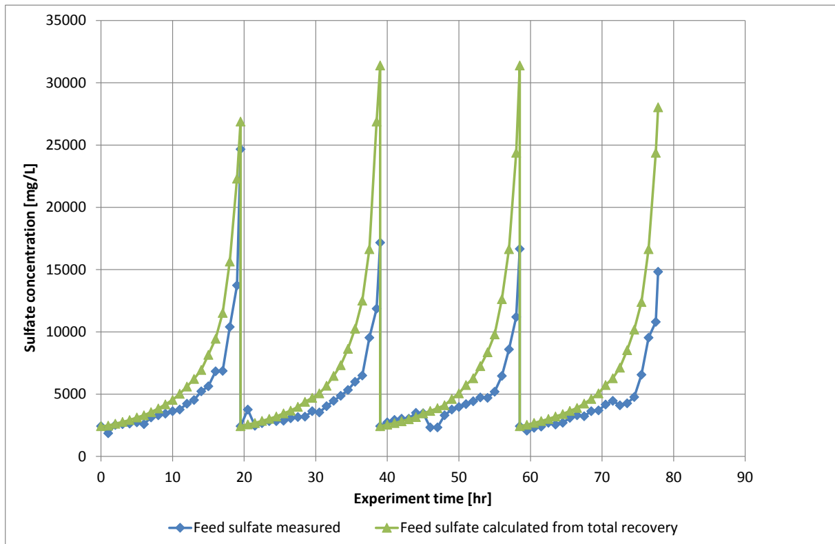
Figure 4: Sulphate Concentration Changes during the Pilot Study
