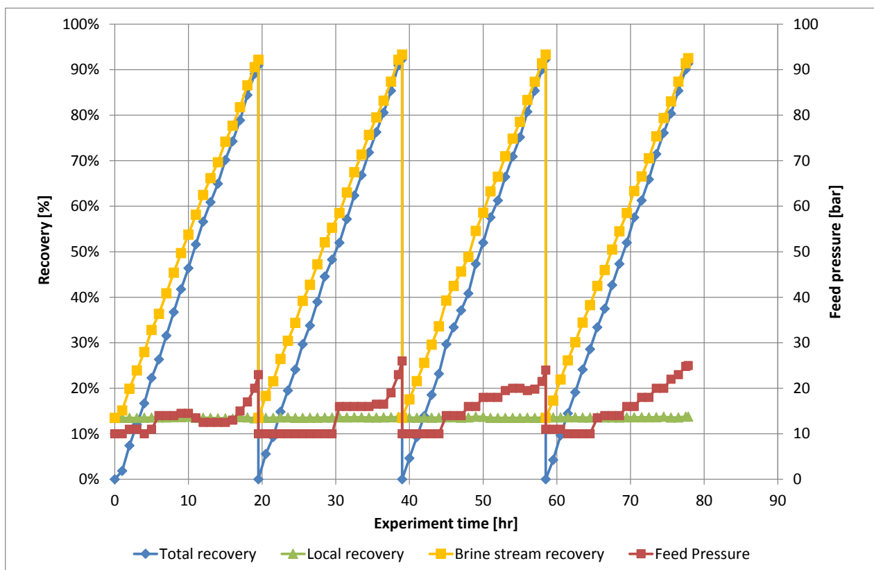
Figure 3: Achieved Recovery and Feed RO Pressure during the Pilot Study
