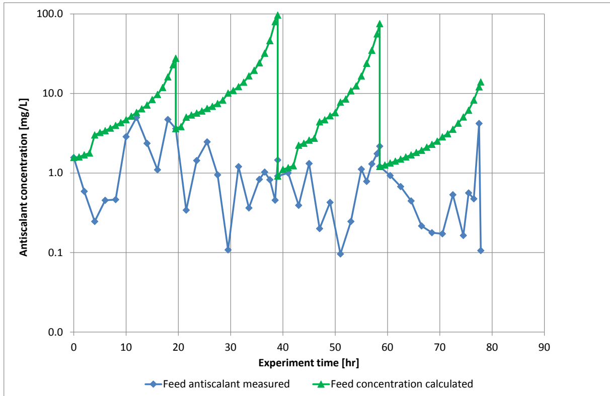
Figure 6: Antiscalant Concentration Changes during the Pilot Study
